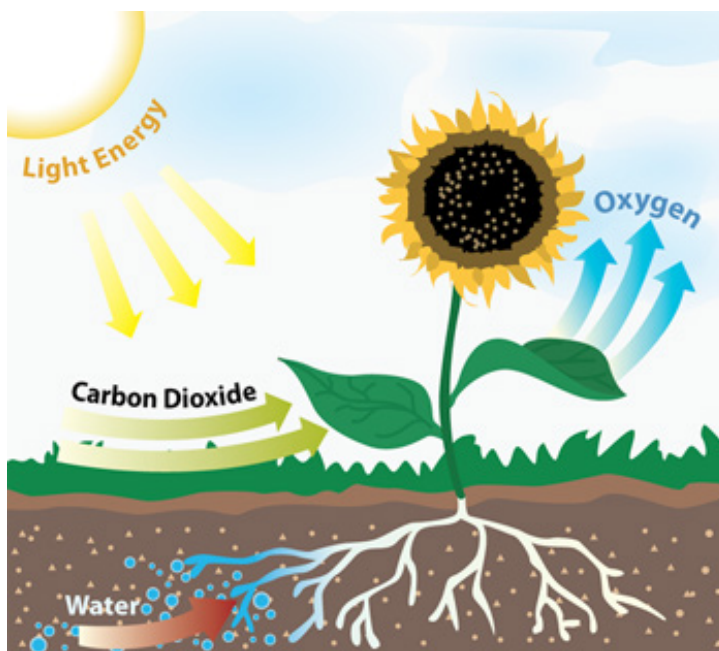
Photosynthesis
